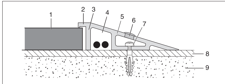
Fig. 5-5: Installation cross-section for Ramp Edge AK 66
