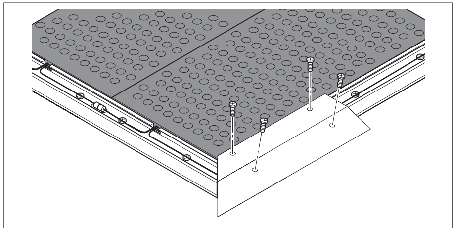
Fig. 5-11: Screw on upper sections of ramp rails
