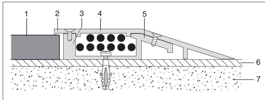
Fig. 5-8: Installation cross-section for Ramp Edges AK 105 and AK 105/1
