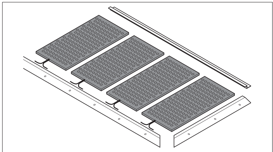
Fig. 5-2: Arrange Safety Mats and fixing rails
