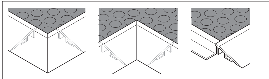
Fig. 5-7: Cut ramp rails on the corners of the Safety Mat system to size
