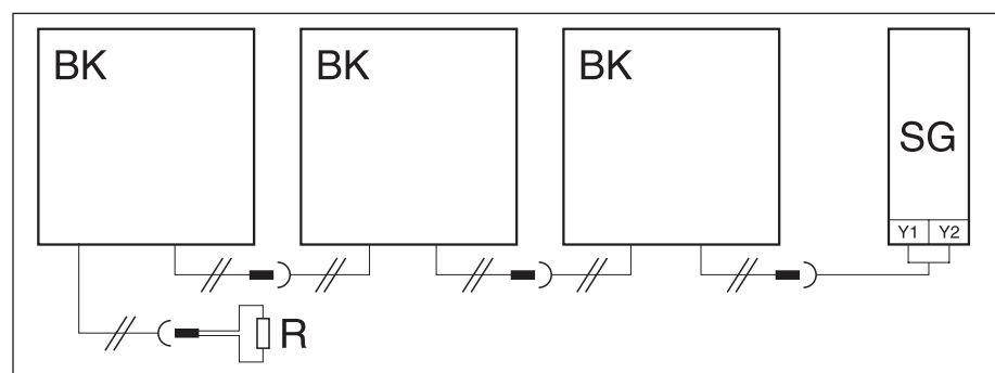
Fig. 5-13: Wiring of Safety Mats BK for 2-wire technology with optional terminal connector, in which the resistor R is integrated
