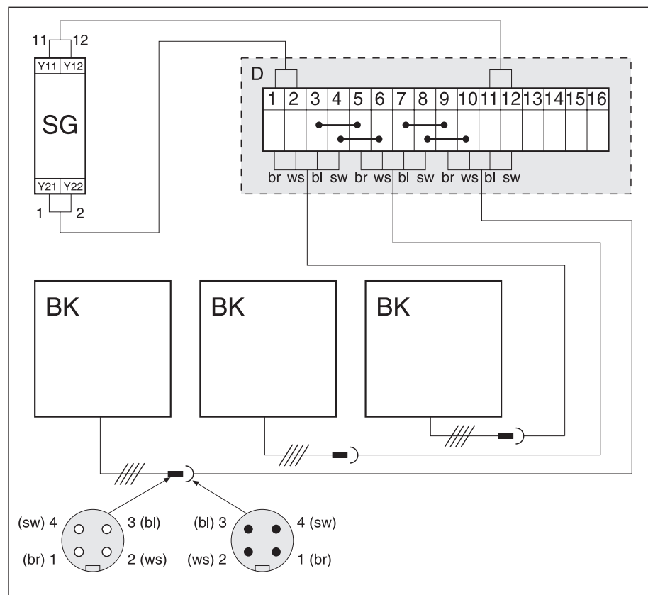
Fig. 5-16: Wiring of the Safety Mats BK for 4-wire technology
