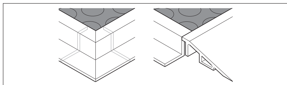
Fig. 5-4: Cut Z-profiles to size for the corners of the Safety Mat system
