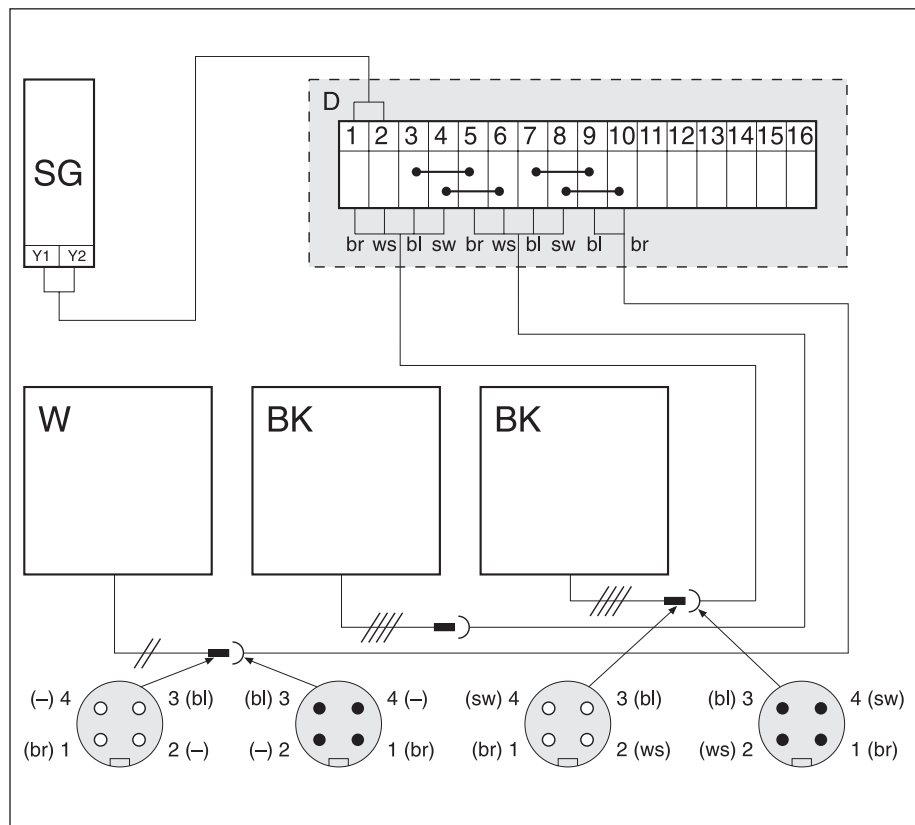
Fig. 5-15: Wiring of the Safety Mats for 2-wire technology
