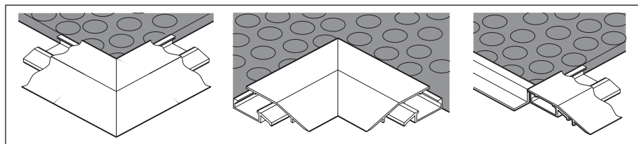
Fig. 5-9: Cut lower sections of the ramp rails on the corners of the Safety Mat system to size
