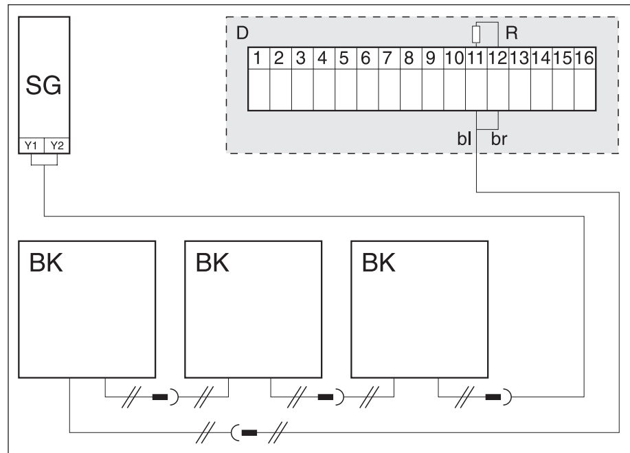
Fig. 5-12: Wiring of the Safety Mats BK for 2-wire technology
