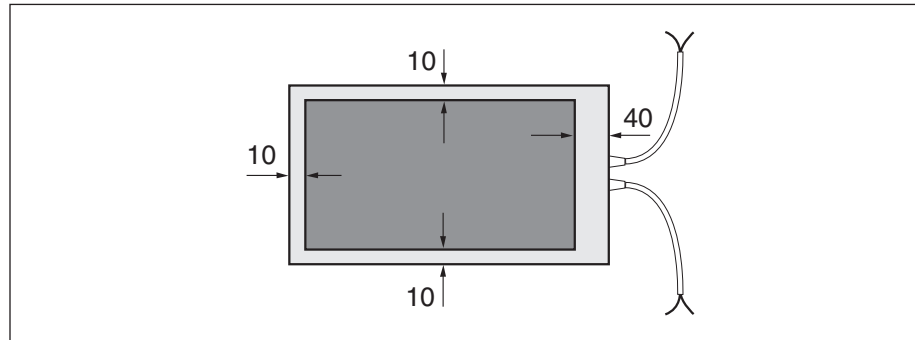
Fig. 2-2: Non-sensitive edges
