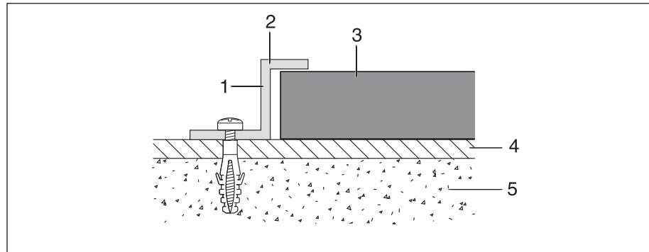
Fig. 5-3: Installation cross-section for Z-profile
