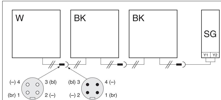
Fig. 5-14: Wiring of the Safety Mats W and BK for 2-wire technology
